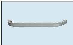
No. 712 Metal D-handle stainless steel-effect drilling distance: 160 mm Projection to the front: 30 mm
