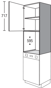
Top-mounted unit for oven
