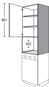
Top-mounted unit for a microwave
