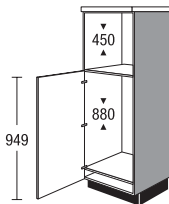
Highboard for built-in appliances
