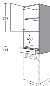
Top-mounted unit for a microwave
