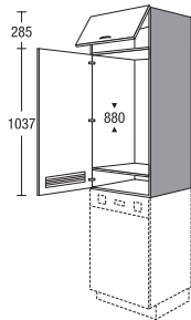
Top-mounted unit for built-in appliance
