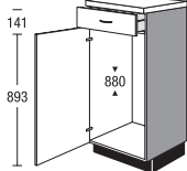
Highboard for built-in appliances
