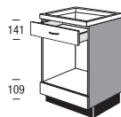
Base unit for a microwave
