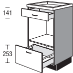
Base unit for built-in appliances
