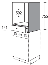
Top-mounted unit for oven
