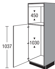
Tall unit for built-in appliances
